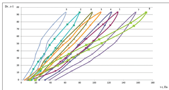
Figure 1: Rheograms of the investigated samples: (1) “Dove Intimo Neutral,” (2) “Lactacyd,” (3) “Femme Intime,” (4) “Nivea intimate,” (5) “Biona Forte,” (6) “Miy Kapriz,” (7) developed gel, (8) “Uriage Gyn Phy”
